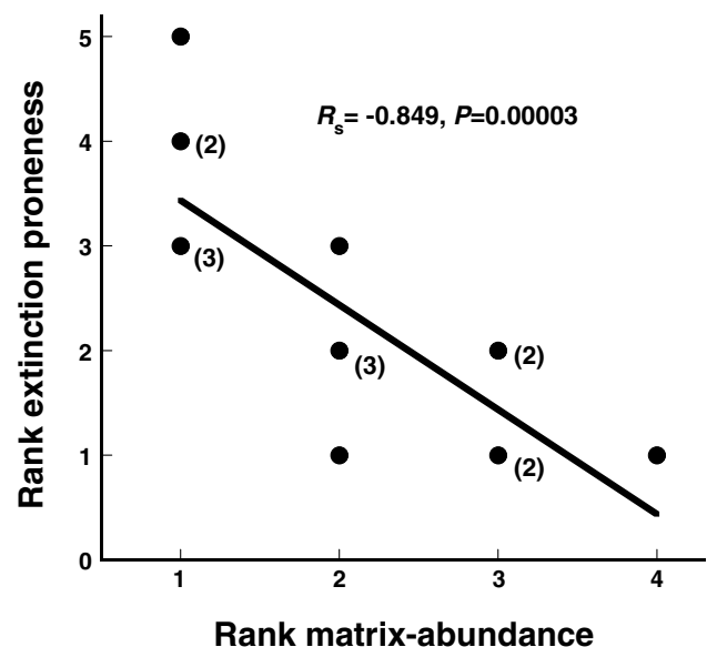
Fig. 4 – Relationship between matrix tolerance and local extinction proneness in 16 mammal species in Australian rainforest fragments (after Laurance, 1991).
